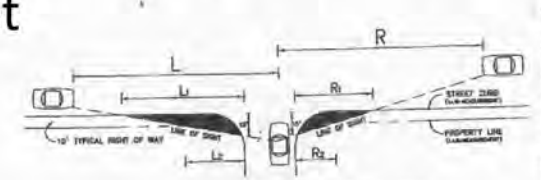
FIGURE C STREETWAY SIGHT DISTANCE REQUIREMENTS
