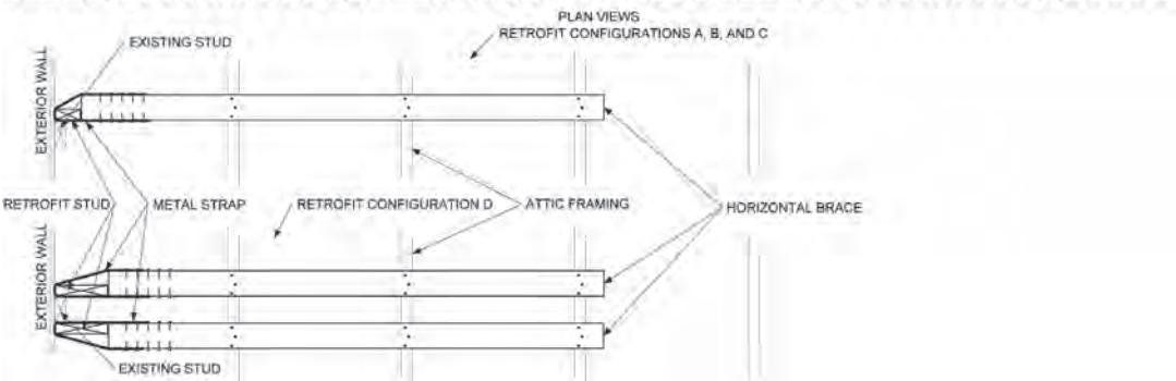
[BS] FIGURE C104.2(3) TRUSS FRAMED GABLE END U-BENT STRAP
