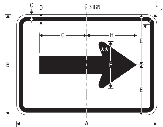
M6-1 DIRECTIONAL ARROW AUXILIARY
