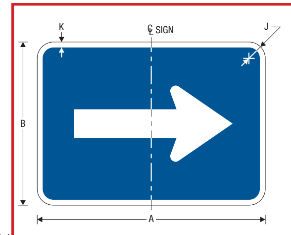
M6-1 DIRECTIONAL ARROW AUXILIARY
